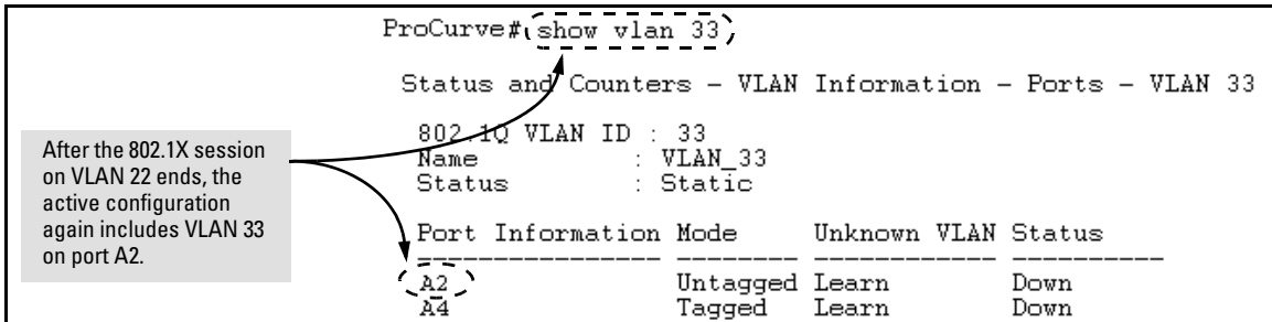
Figure 12-22. The Active Configuration for VLAN 33 Restores Port A2 After the 802.1X Session Ends
